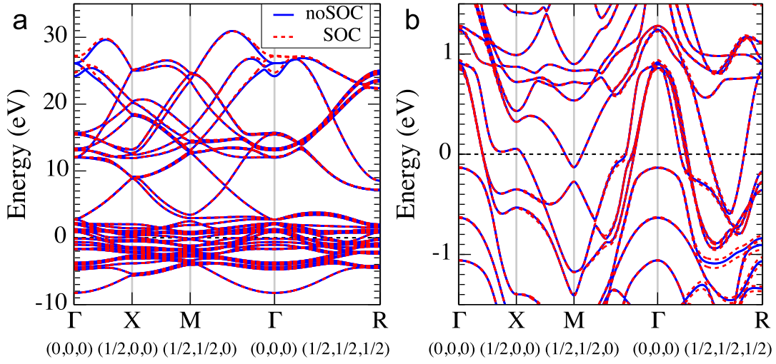
Supplementary Figure 1. Band structures of \gamma -Fe 0.5 Mn 0.5 . a Band structures of \gamma -Fe 0.5 Mn 0.5 without and with spin-orbit coupling under the strain \delta=0.95 . b The enlarged band structures within the energy range of [-1.5\sim 1.5] eV. The bands are twofold spin degenerate unless the spin-orbit coupling is switched on.
