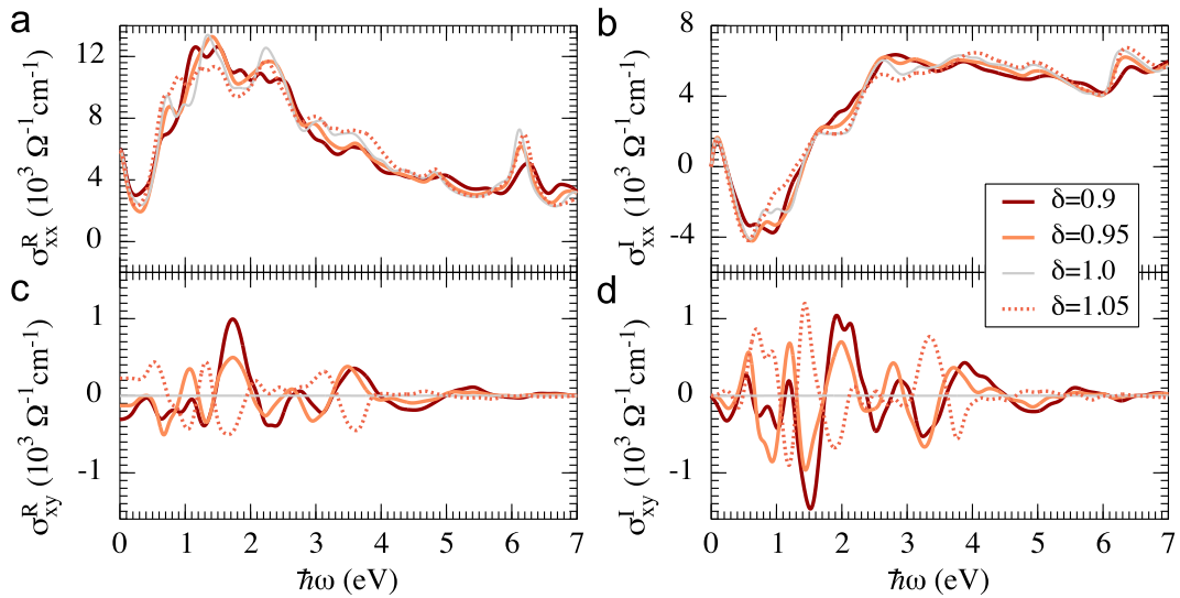
Supplementary Figure 2. The optical conductivities of \gamma -Fe 0.5 Mn 0.5 under various strains. a,b The diagonal elements have similar profiles regardless of strains. The Drude term has been added to the diagonal elements. c,d The off-diagonal elements (i.e., the magneto-optical conductivity) arise only after the strains are applied. In particular, the magneto-optical conductivity can be effectively tuned by the strain, that is, the magnitude of \sigma_{xy}(\omega) is proportional to |\delta - 1| and the sign of \sigma_{xy}(\omega) changes along with \text{sgn}(\delta - 1) . The spin-orbit coupling is not included in the calculations.
