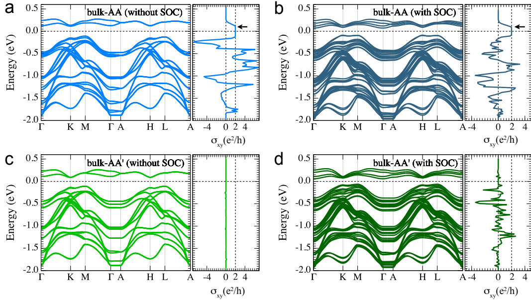
Supplementary Figure 4. The band structures and anomalous Hall conductivities of K 0.5 RhO 2 . a,b The band structures and anomalous Hall conductivities of the AA stacked K 0.5 RhO 2 without and with spin-orbit coupling. c,d The same as a,b but for the AA' stacked K 0.5 RhO 2 . The bands are twofold spin degenerate without spin-orbit coupling. The AA stacked K 0.5 RhO 2 is a quantum topological Hall insulator with the Chern number C=2 . On the other hand, the AA' stacked K 0.5 RhO 2 is a normal insulator with the Chern number C=0 . The anomalous Hall conductivities of K 0.5 RhO 2 are scaled by the length of the crystallographic z axis such that the unit is e^2/h in accord with that of two-dimensional systems.
