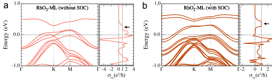
Supplementary Figure 5. The band structures and anomalous Hall conductivities of RhO 2 monolayer. a The band structures and anomalous Hall conductivities of RhO 2 monolayer without spin-orbit coupling. b The same as a but with spin-orbit coupling. The bands are twofold spin degenerate without spin-orbit coupling. RhO 2 monolayer is metallic intrinsically. However, it turns out to be a quantum topological Hall insulator with the Chern number C=1 , if the Fermi energy is moved into the band gap above, e.g., by electron doping.
