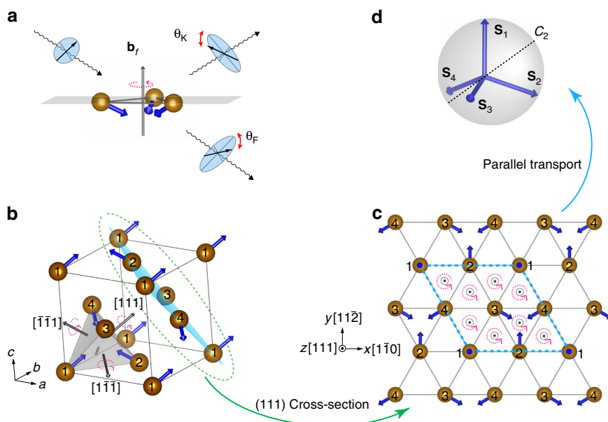
Fig. 1 Topological light-matter interactions in chiral magnets. a Sketch of topological light-matter interactions in a minimal chiral magnet comprising three neighboring noncoplanar spins. \mathbf{b}_f is the fictitious magnetic flux generated by the finite scalar spin chirality. Topological magneto-optical Kerr and Faraday effects are induced by the fictitious magnetic flux \mathbf{b}_f rather than by the nonzero net magnetization. b The 3Q noncoplanar antiferromagnet on a 3D fcc lattice. The numbers 1–4 label the four magnetic sublattices, which are the corners of a tetrahedron (gray color). Blue and gray arrows indicate the directions of the localized spin \mathbf{S}_i and the fictitious magnetic flux \mathbf{b}_f , respectively. c The 3Q nc-AFM on a 2D triangular lattice. It is the (111) cross-section of the 3D fcc lattice, indicated by cyan color in b . Dashed cyan lines mark the 2D unit cell. \odot indicate the directions of the \mathbf{b}_f on each triangular plaquette. d The unit sphere is spanned by the spins on four sublattices that are parallel transported to have a common origin. The dashed line indicates one of the C_2 rotation axes in spin space.
