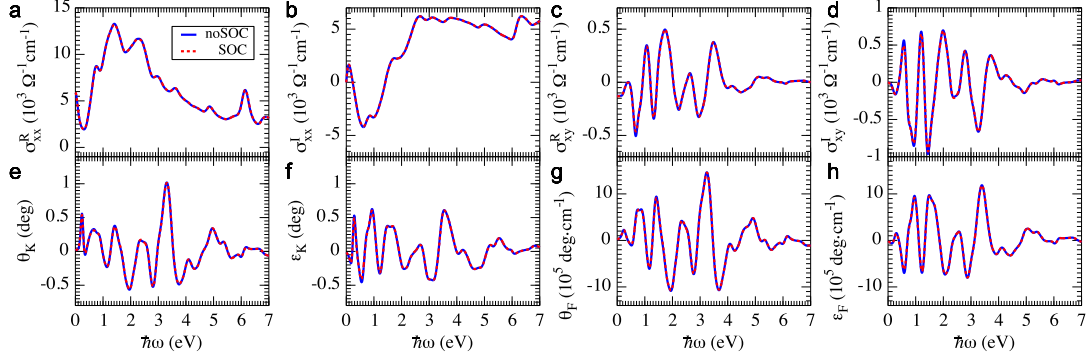
Supplementary Figure 3. The optical conductivity and magneto-optical spectrum of \gamma -Fe 0.5 Mn 0.5 . The optical conductivity a-d as well as the magneto-optical Kerr e,f and Faraday g,h spectra without and with spin-orbit coupling. The Drude term is included and the strain \delta=0.95 is applied along the [111] direction. Spin-orbit coupling does not influence the magneto-optical effects in \gamma -Fe x Mn 1-x , demonstrating the topological origin of magneto-optical effects.
